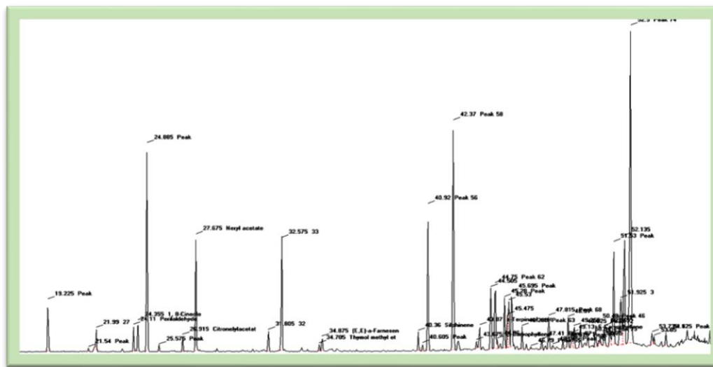
Figure 2. Chromatogram of Illicium Verum fruits Essential oils
